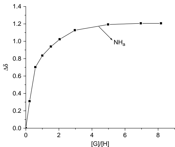
Figure 8. Titration curve for 1 ( c = 1.86 \times 10^{-3} M) with tetrabutylammonium salt of benzoate.
