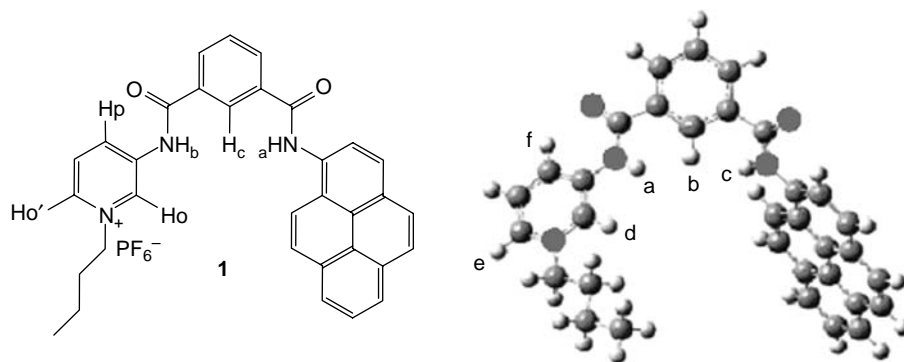
Figure 1. Density functional theory-optimised structure of 1 ( E = -1589.33 au; atomic charges: a = 0.2485 , b = 0.0735 , c = 0.2314 , d = 0.1707 , e = 0.1669 , f = 0.1902 , N^+ = -0.3792 ).
