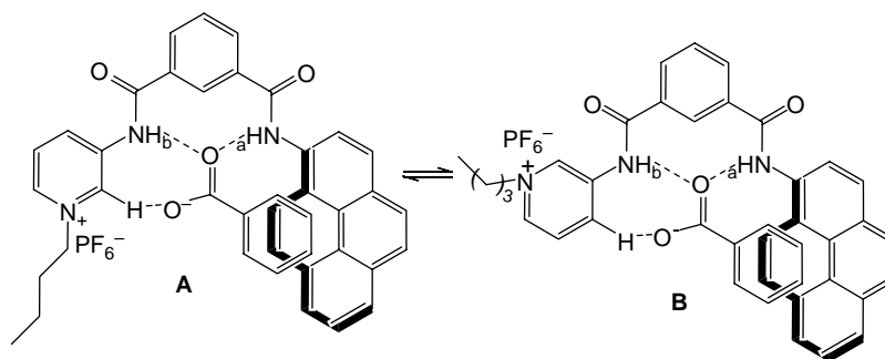
Figure 7. Suggested mode of binding of C_6H_5CO_2^- into the cleft of 1 .
